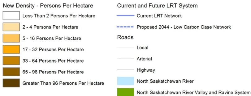
Low Carbon Case - 2044 New Density - Persons Per Hectare
