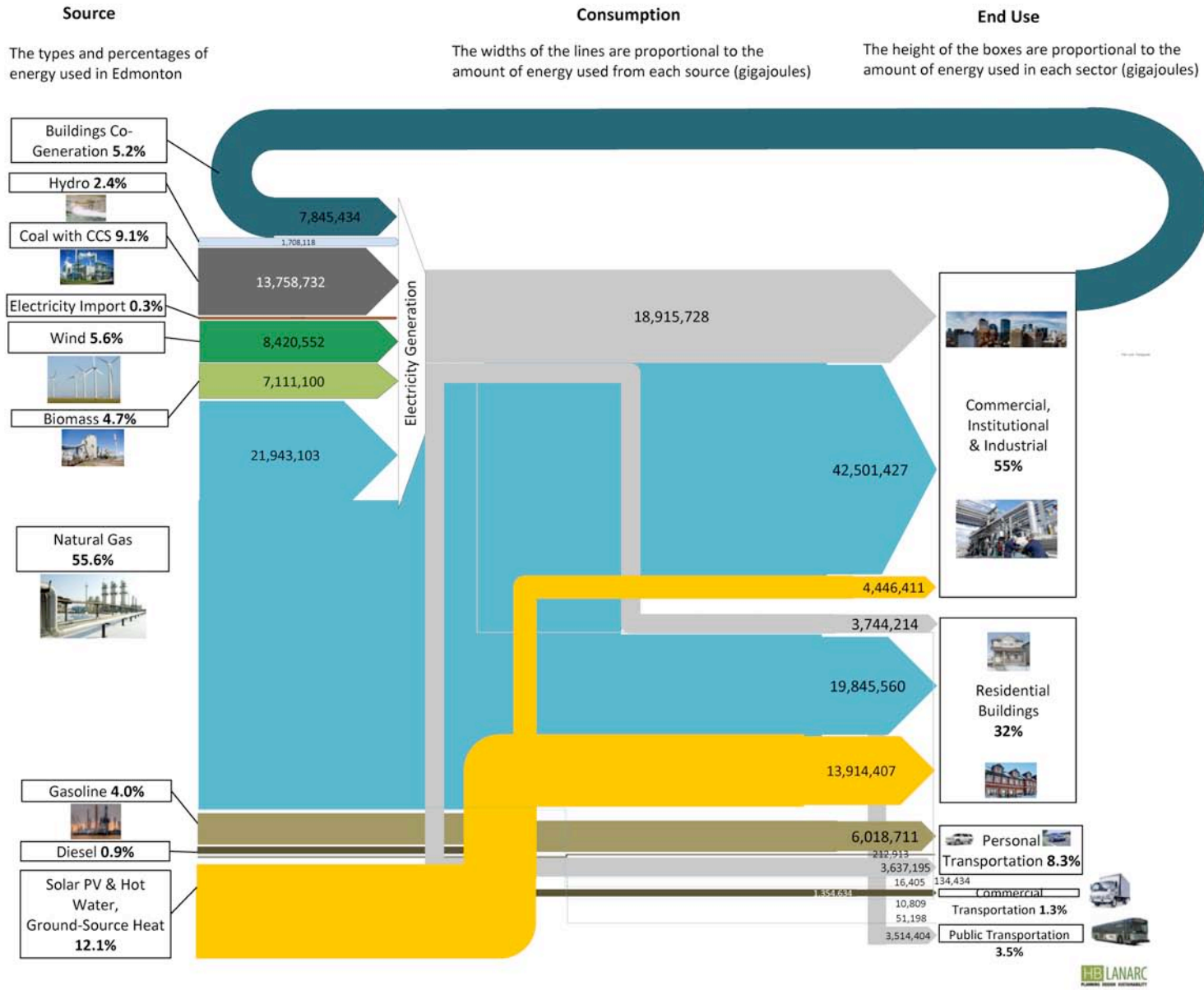
Figure 9: Energy supply and use in Edmonton (2044) – Low Carbon Case, excluding heavy industry
